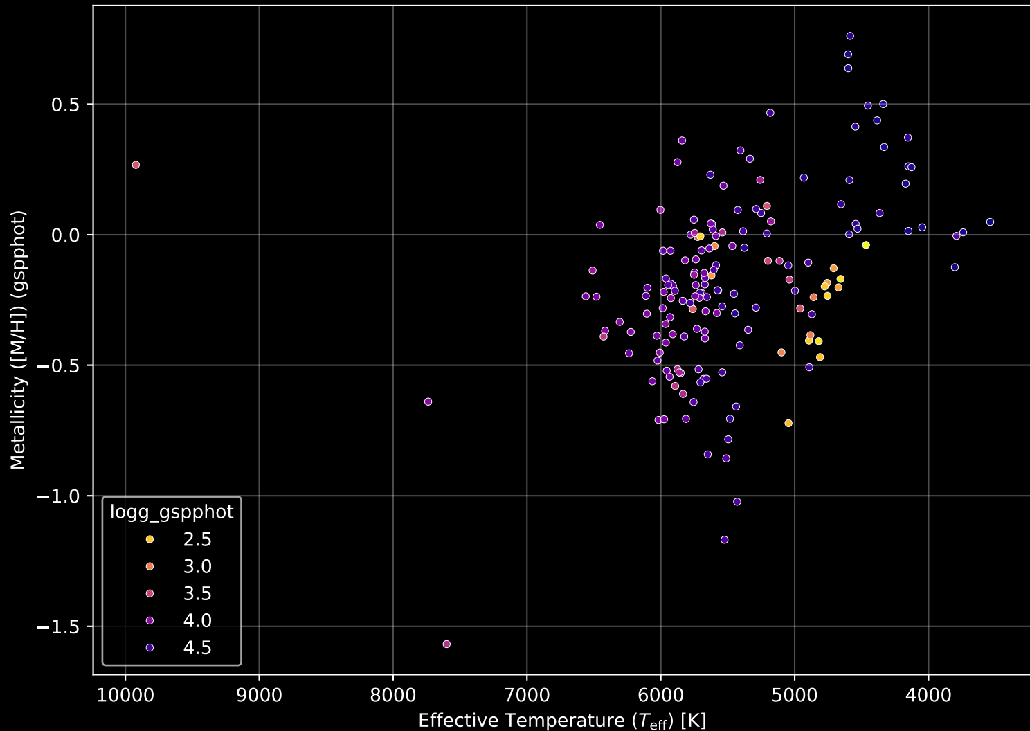
APOGEE DR17 Field: [063+88_MGA] Stellar Population Parameters (n= 170)
