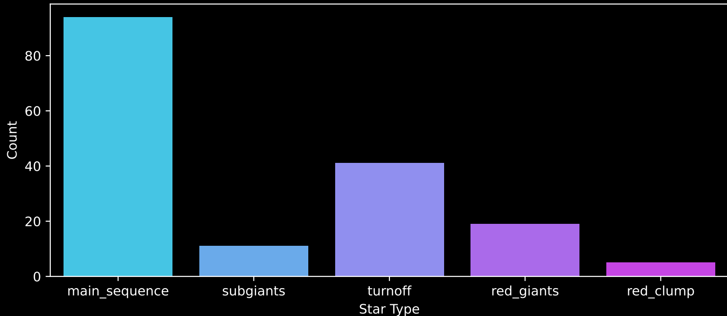
APOGEE DR17 Field: [063+88_MGA] Count plot of Star Type
