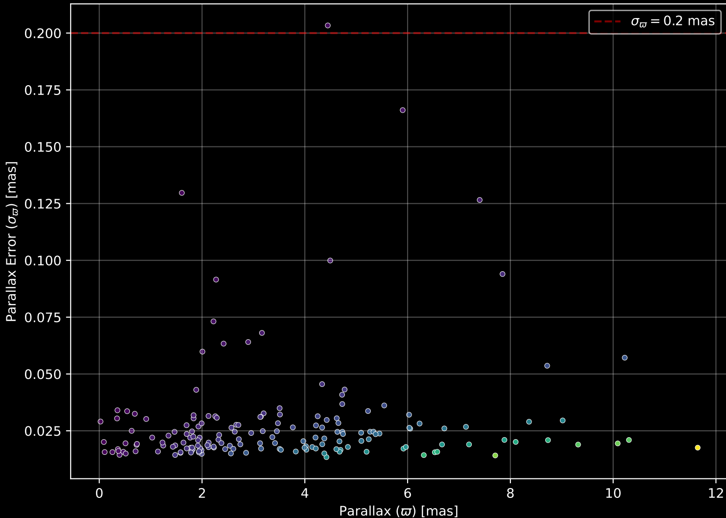
APOGEE DR17 Field: [063+88_MGA] Parallax Quality (n= 170)
