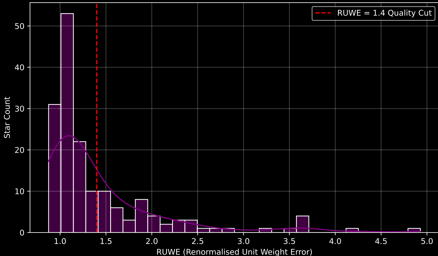
GAPOGEE DR17 Field [063+88_MGA] RUWE Distribution (n= 166)
