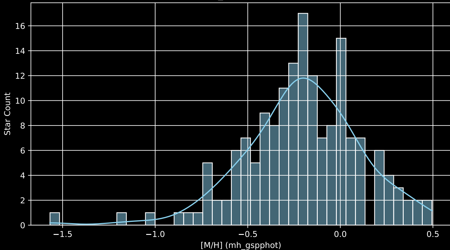
APOGEE DR17 Field: [063+88_MGA [M/H] (mh_gspphot) (n= 166)
