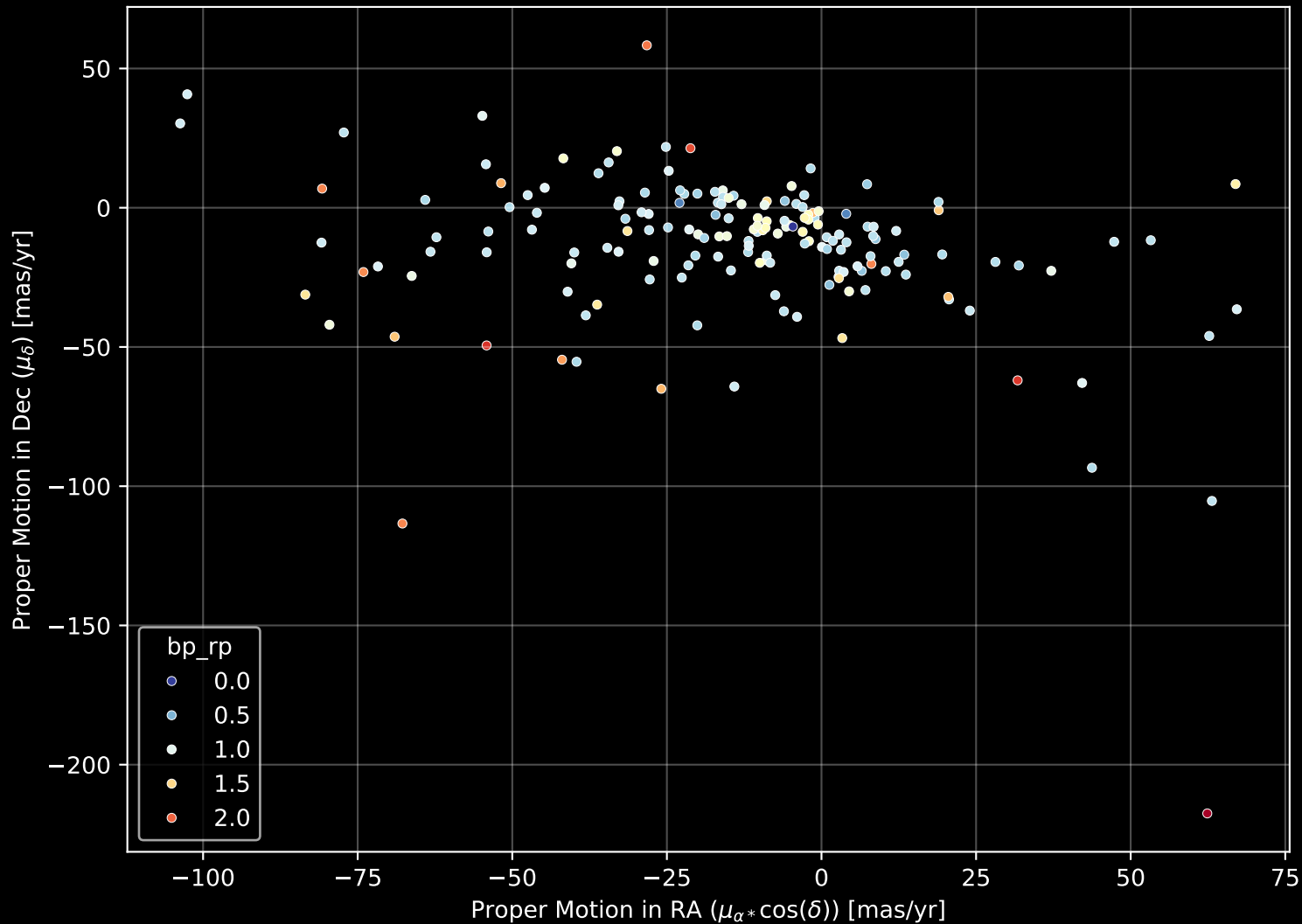
APOGEE DR17 Field: [063+88_MGA] Proper Motion Diagram (n= 170)
